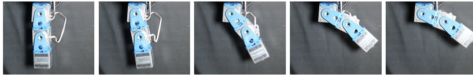
Fig. 4. Photo-sequence of the the last iteration of the slow minimum jerk trajectory in the heavy payload scenario.
